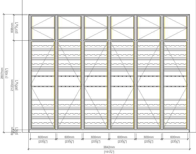
Elevation C
